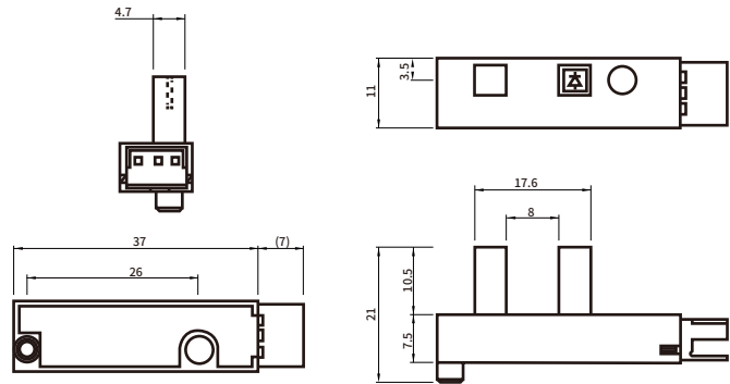
Dimensions (mm)
